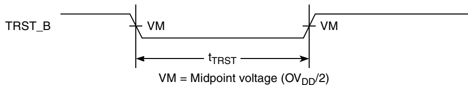
Figure 24. TRST_B Timing Diagram
