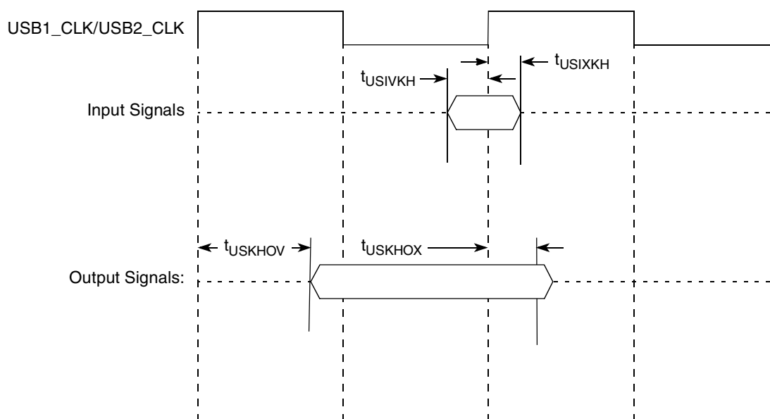
Figure 16. USB Signals
