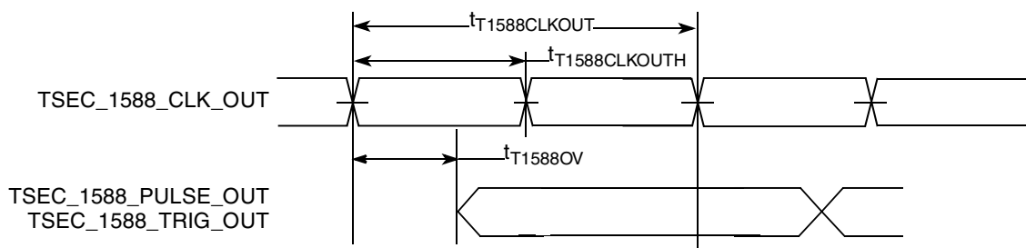
Figure 13. dTSEC IEEE 1588 Output AC Timing
