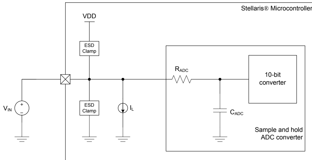
Figure 26-13. ADC Input Equivalency Diagram
