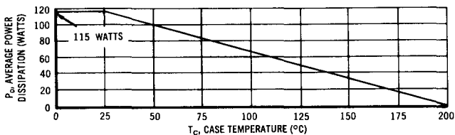
FIGURE 1 — POWER DERATING CURVE
