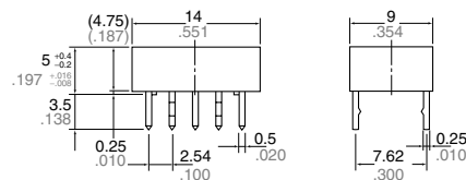
Self-clinching terminal
