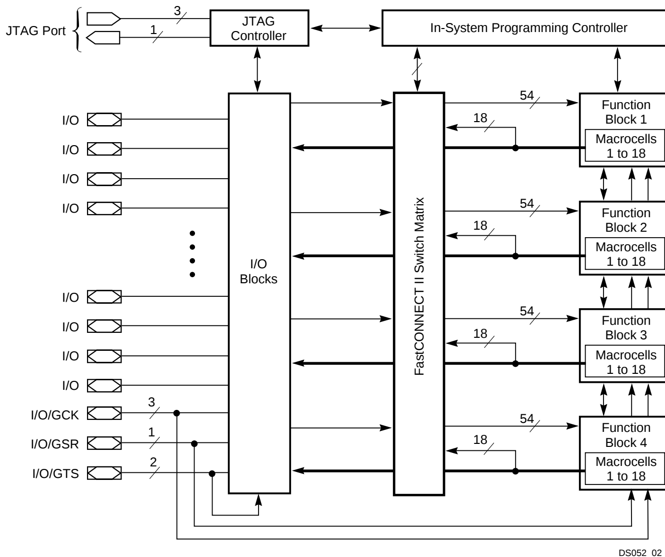
Figure 2: XC9572XV Architecture
