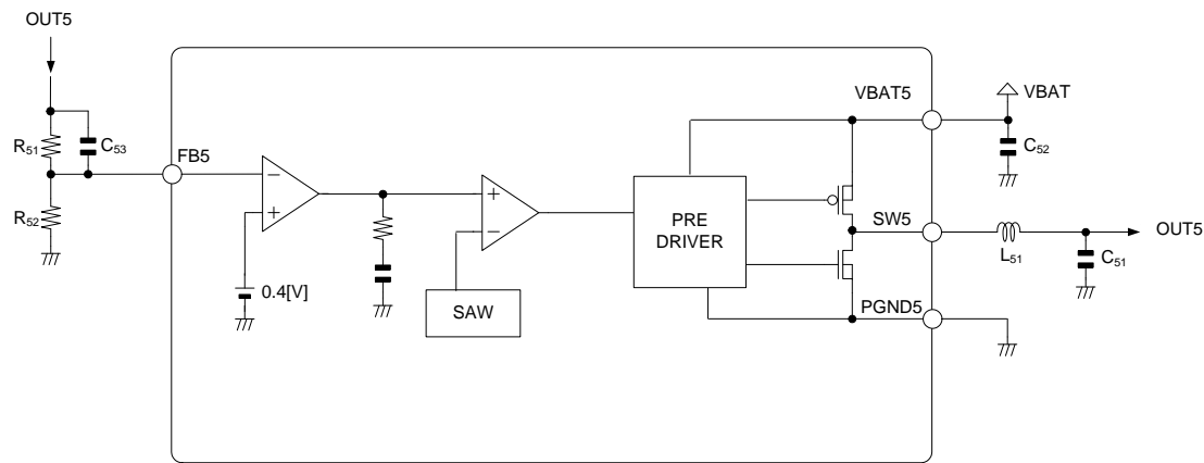
(b) Recommended External Components
