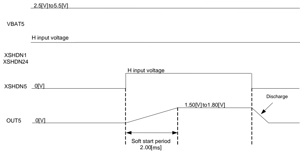
(c) Start-up Sequence
