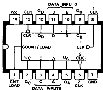
B138 SN74196N 50 MHz decade counter
