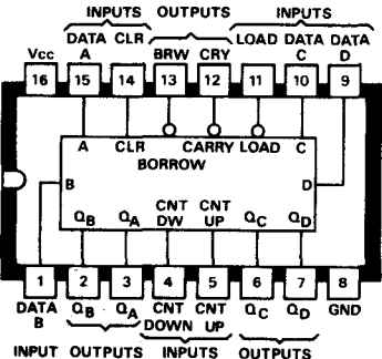
B135 SN74193N SN74L193N/SN74C193N Up/Down binary counter
