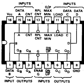
B134 SN74192N SN74L192N/SN74C192N Up/Down decade counter
