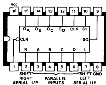
B137 SN74195N SN74C195N 4-bit shift register
