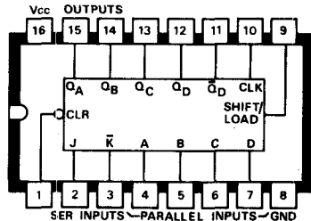
B137 SN74195N SN74C195N 4-bit shift register
