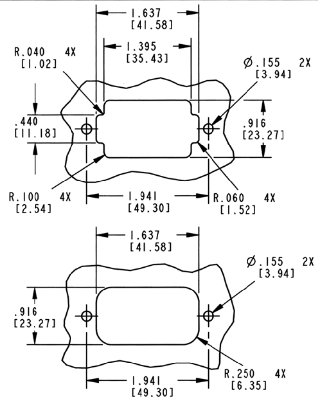
RECOMMENDED PANEL CUTOUTS
