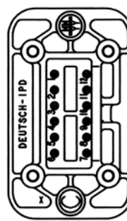
DT15-12PC-G003 COLOR GREEN
