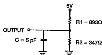
(c) Three-State Delay (Load 3)
