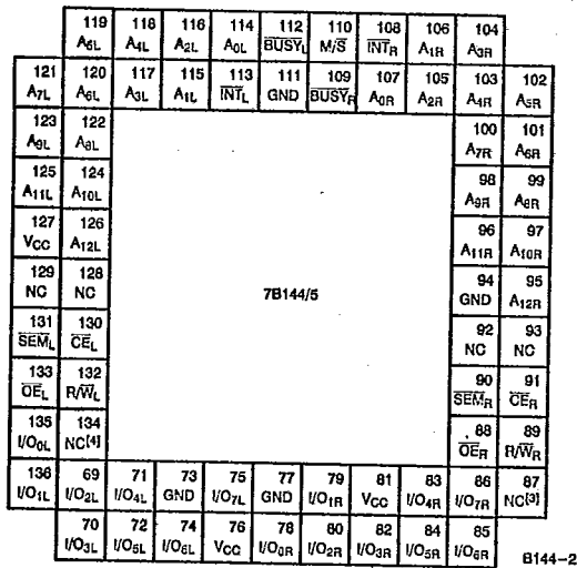
68-Pin PGA Top View
