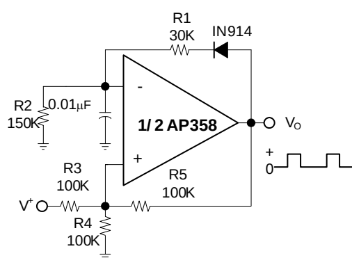
Pulse Generator
