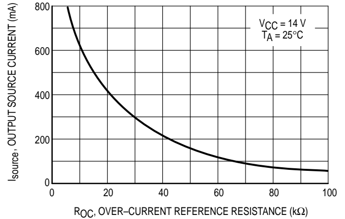
Figure 8. Output Source Current–Limit versus Over–Current Reference Resistance
