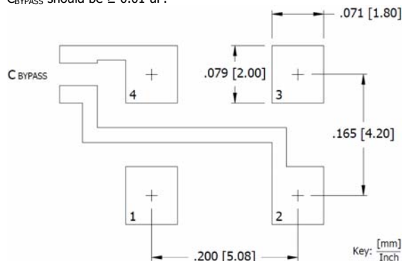
SUGGESTED SOLDER PAD GEOMETRY
