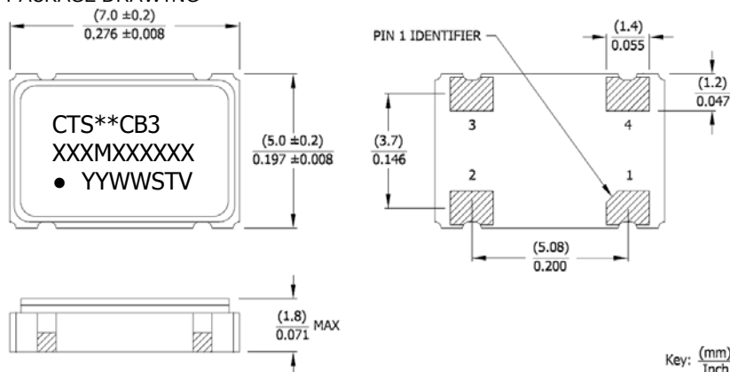
PACKAGE DRAWING
