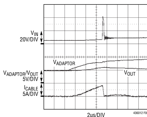
FIGURE 5 CIRCUIT R_{IN} = 150\mu\Omega , L_{IN} = 2\mu H LOAD = 10\Omega , C_{OUT} = 10\mu F
