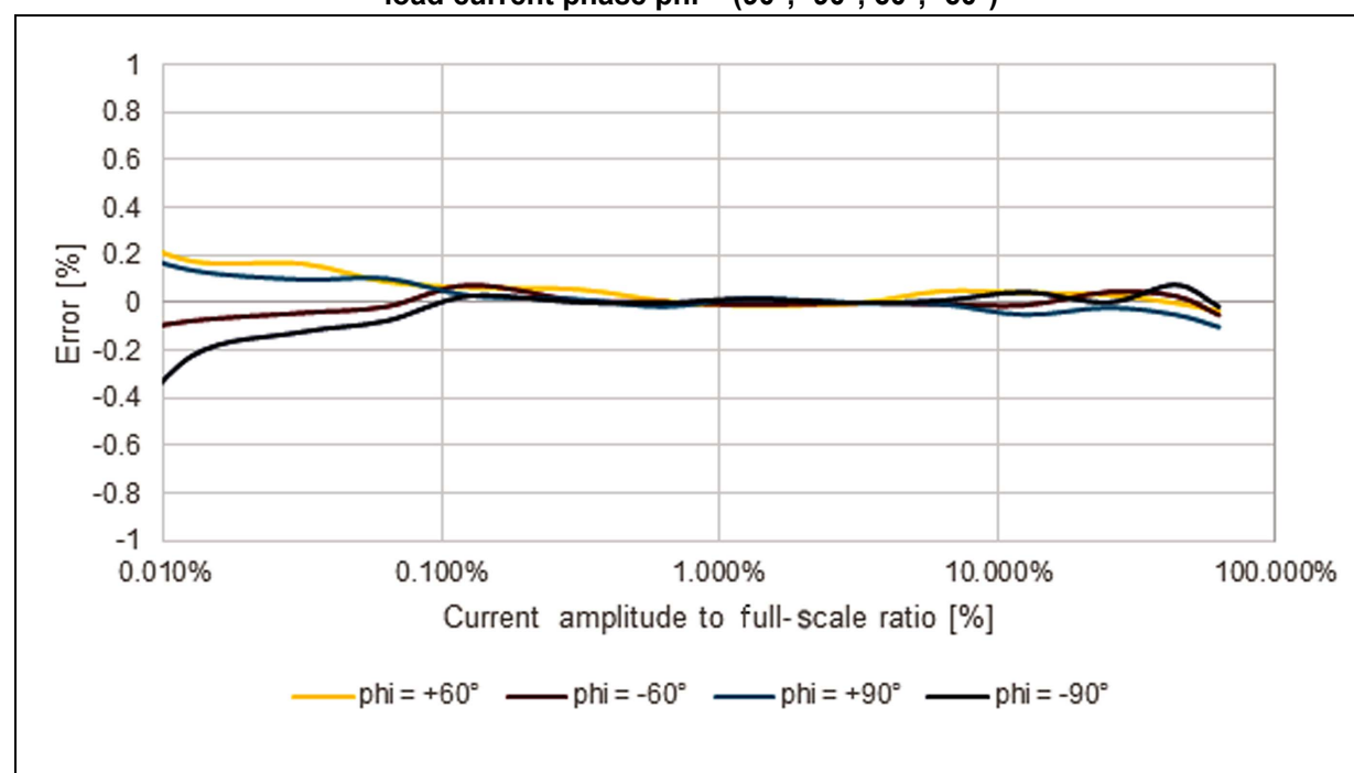
Figure 16. Reactive energy error vs. current at A_I = 2x , T = 25\text{ }^{\circ}\text{C} , load current phase \phi = (90^{\circ}, -90^{\circ}, 60^{\circ}, -60^{\circ})
