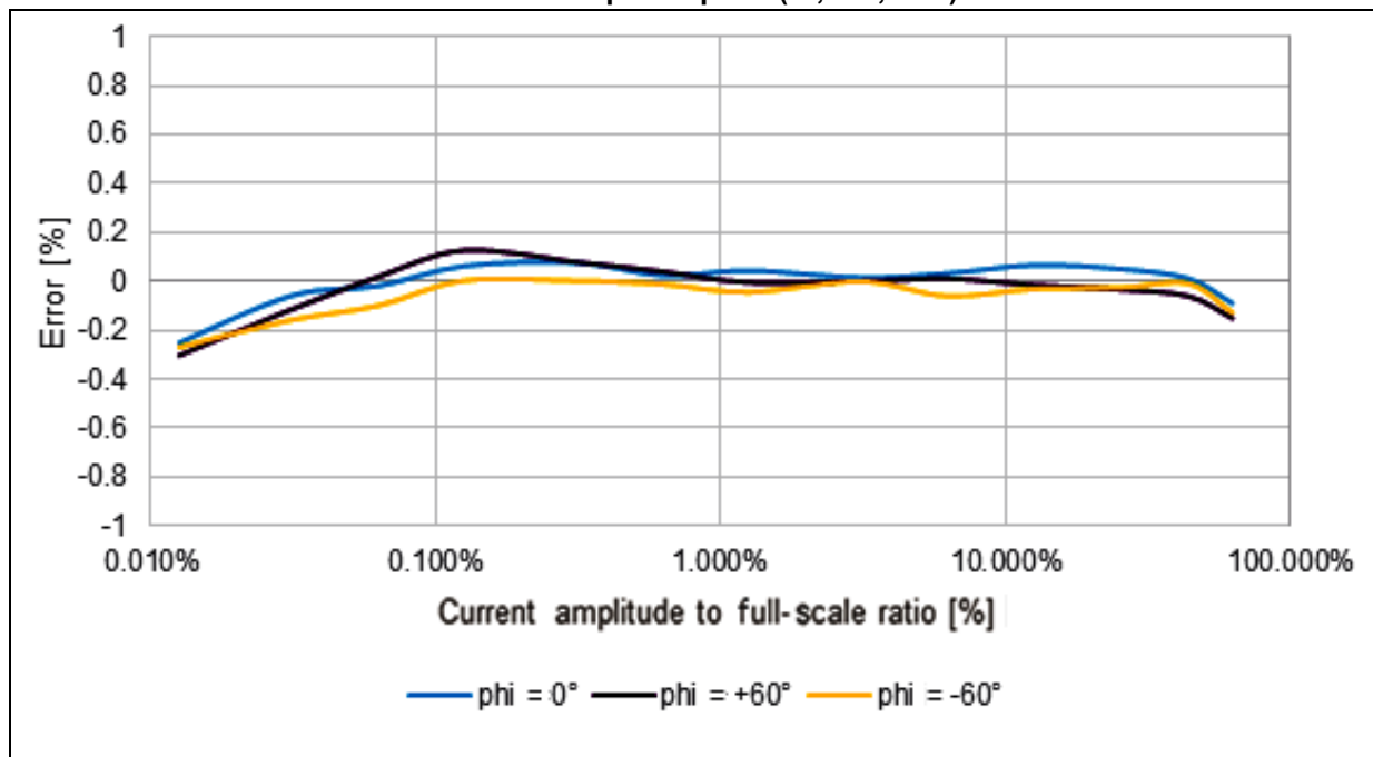
Figure 12. Active energy error vs. current at A_I = 16x , T = 25\text{ }^{\circ}\text{C} , load current phase \phi = (0^{\circ}, 60^{\circ}, -60^{\circ})
