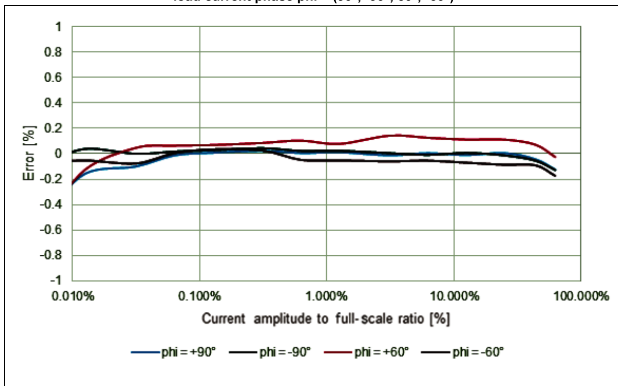
Figure 17. Reactive energy error vs. current at A_I = 16x , T = 25\text{ °C} , load current phase \phi = (90^\circ, -90^\circ, 60^\circ, -60^\circ)
