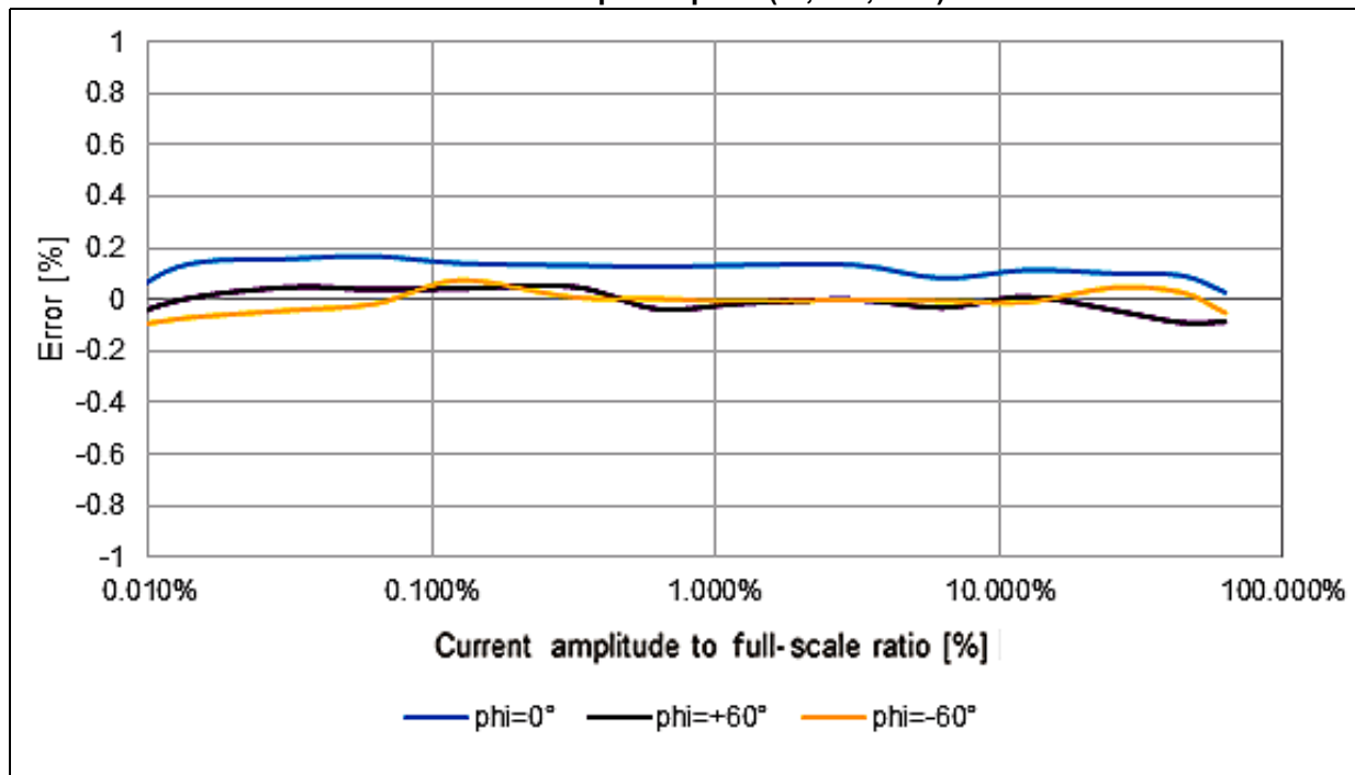
Figure 12. Active energy error vs. current at A_I = 16x , T = 25\text{ }^{\circ}\text{C} , load current phase \phi = (0^{\circ}, 60^{\circ}, -60^{\circ})
