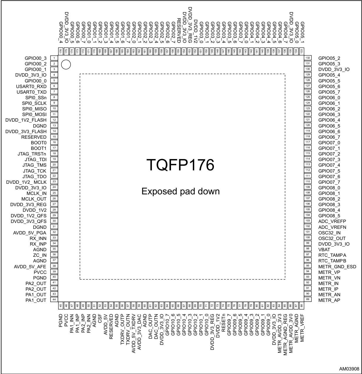
Figure 7. TQFP176 pinout
