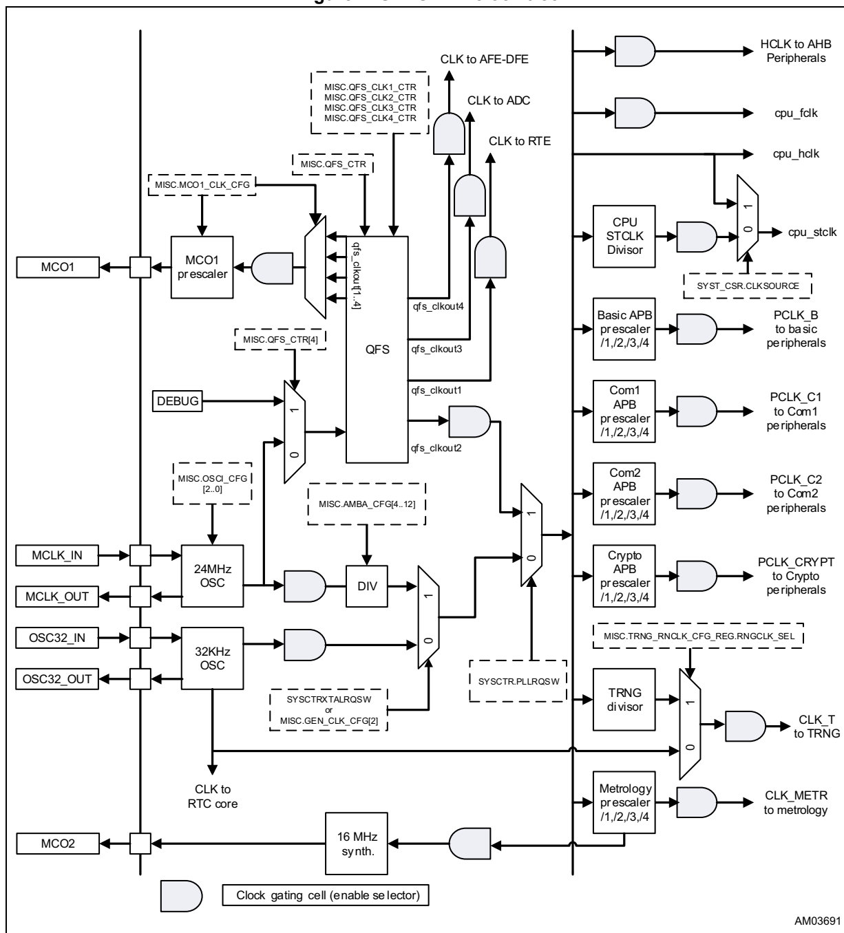
Figure 4. STCOMET clock tree
