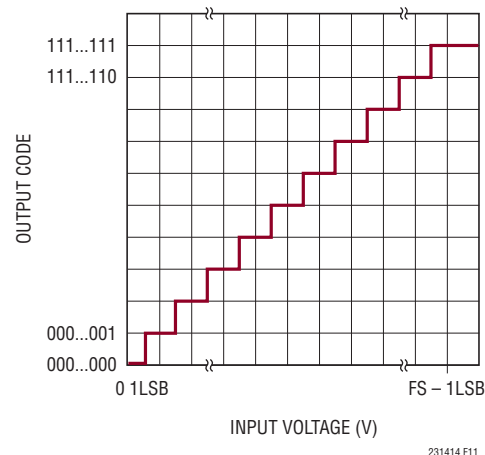
Figure 11. LTC2314-14 Transfer Function
