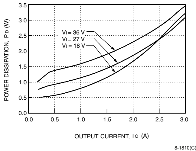
Figure 51. LC010F Typical Power Dissipation vs. Output Current at T_c = 25^\circ\text{C}
