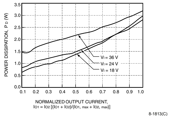
Figure 52. LC010AJ, BK, CL Typical Power Dissipation vs. Normalized Output Current at T_c = 25^\circ\text{C}
