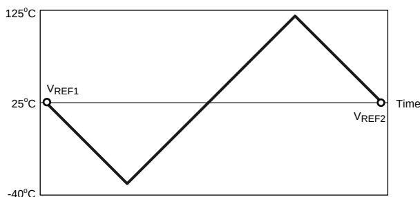
Figure 47. Temperature Profile
