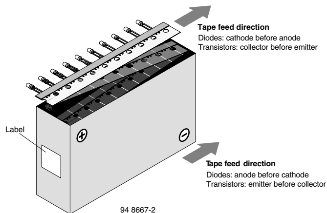
Fig. 31 - Tape Direction
