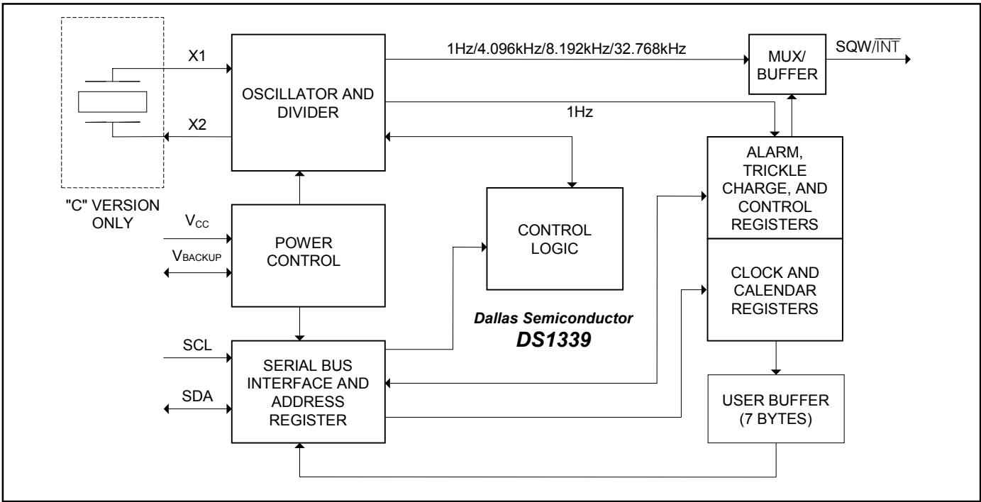
Figure 3. Block Diagram
