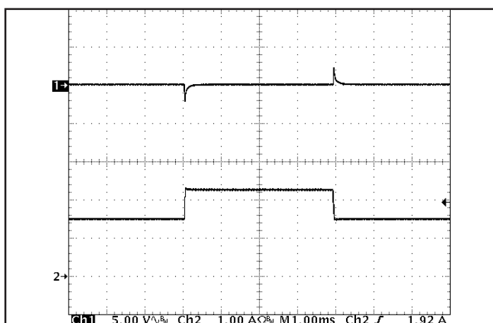
Figure 5: Output voltage response to step-change in load current (50%-75%-50% of I_{out(max)} ; dI/dt = 0.1A/\mu s ). Load cap: 15 \mu F tantalum cap and 1 \mu F ceramic cap. Ch 1: V_{out} , Ch 2: I_{out} .
