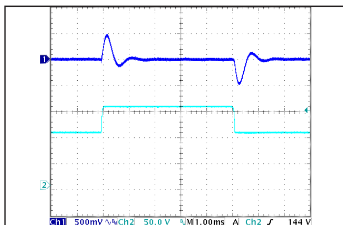
Figure 6: Output voltage response to step-change in input voltage (nominal to maximum input voltage), at Full Load current. Load cap: 1 \mu F ceramic cap. Ch 1: V_{out} , Ch 2: V_{in} .
