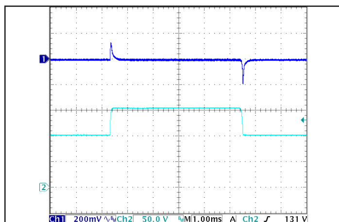
Figure 6: Output voltage response to step-change in input voltage (nominal to maximum input voltage), at Full Load current. Load cap: 15μF tantalum capacitor and 1uF ceramic cap. Ch 1: V out , Ch 2: V in .
