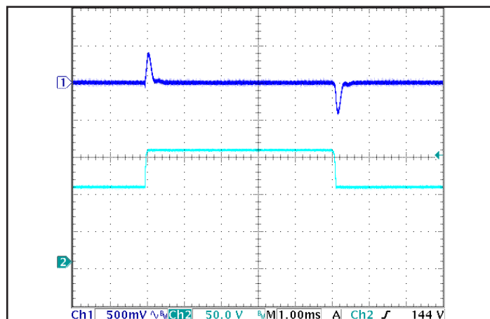
Figure 6: Output voltage response to step-change in input voltage (nominal to maximum input voltage), at Full Load current. Load cap: 1uF ceramic cap. Ch 1: Vout, Ch 2: Vin.
