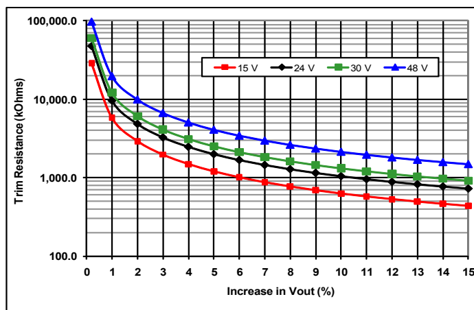
Common Figure 3: Trim-Up Graph for 15 to 48V outputs.
