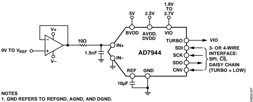
Figure 23. Typical Application Diagram with Multiple Supplies
