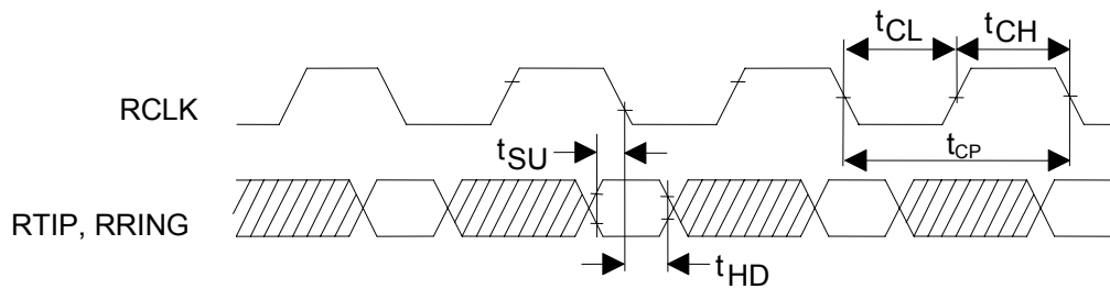
Figure 12-7. Receive Framing Timing—Line Side
