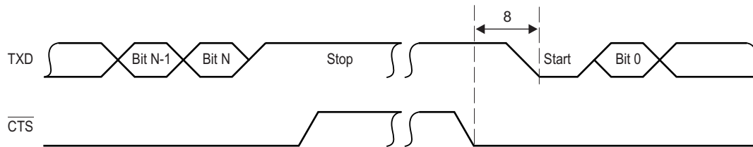
Figure 11-40. UART CTS (Clear-to-Send Input) — Autoflow Timing Waveform
