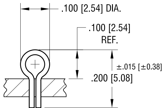
SHOWN AS INSTALLED INTO .040 [1.02] DIA. MOUNTING HOLE
