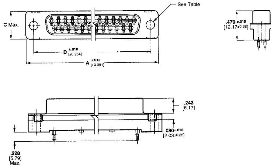
With Standard Mounting Holes
