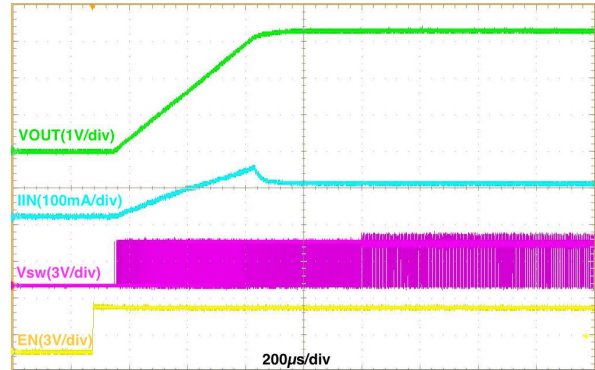
Figure 25. Start-up, V_{IN} = 3.6\text{ V} , V_{OUT} = 3.3\text{ V} , 100 mA Resistive Load, Auto Mode
