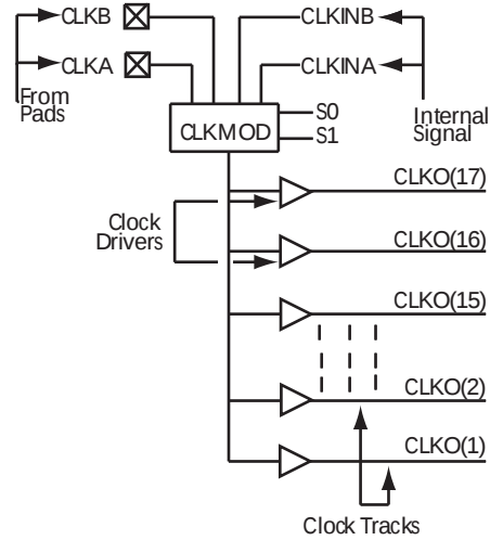
Figure 1-7 • Clock Networks of 42MX Devices
