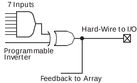
Figure 1-4 • A42MX24 and A42MX36 D-Module Implementation
