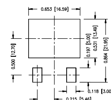
Min. Recommended Footprint
