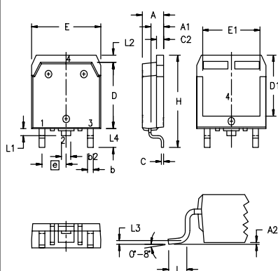
TO-268AA (IXST) (D 3 PAK)
