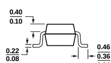
Figure 35. 5-Lead Thin Shrink Small Outline Transistor Package [SC70] (KS-5)
