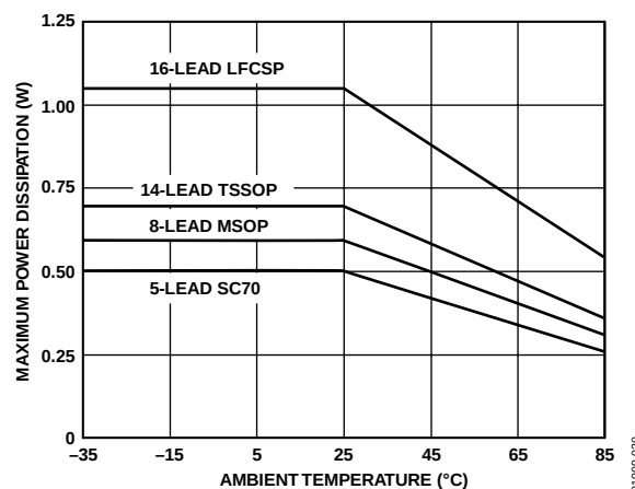
Figure 30. Maximum Power Dissipation vs. Temperature for 5-Lead SC70, 8-Lead MSOP, 14-Lead TSSOP, and 16-Lead LFCSP Packages
