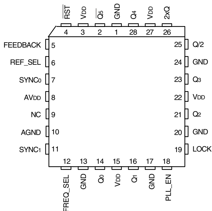
PLCC TOP VIEW
