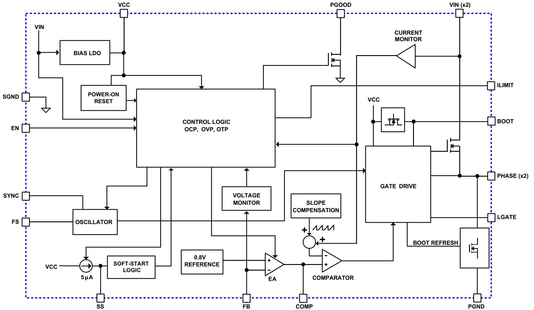
FIGURE 3. BLOCK DIAGRAM
