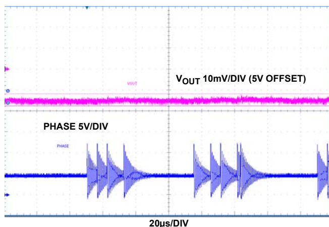
FIGURE 18. NON-SYNCHRONOUS BUCK, FORCE PWM MODE, V_{IN} 12V, NO LOAD
