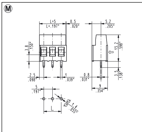
MSM_001 - 000T 5 mm / .197" Pitch
