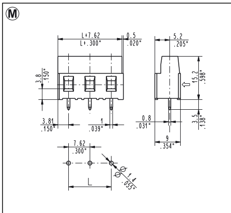
MSM_007 - 000T 7.62 mm / .300" Pitch
