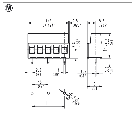
MSM_002 - 000T 10 mm / .394" Pitch
