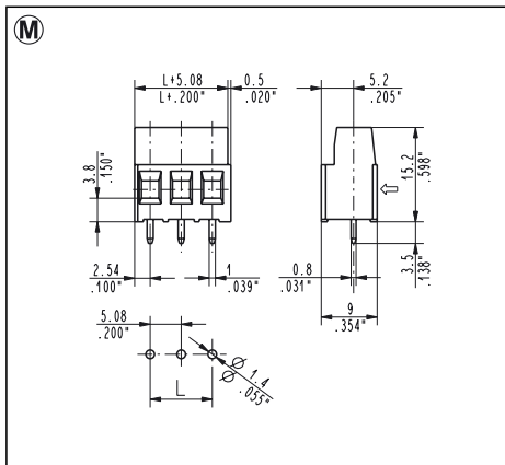
MSM_005 - 000T 5.08 mm / .200" Pitch
