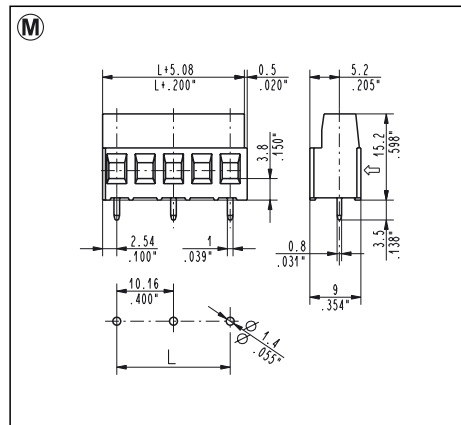
MSM_006 - 000T 10.16 mm / .400" Pitch
