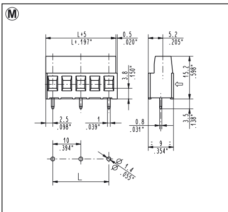
MSM__002 Straight, Side Entry 10 mm / .394" Pitch Weight per pole: 1.77 g
