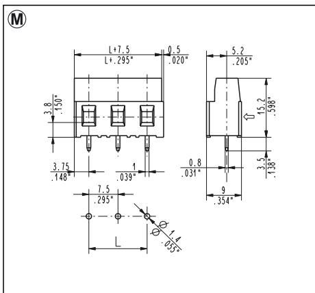
MSM_003 - 000T 7.5 mm / .295" Pitch
