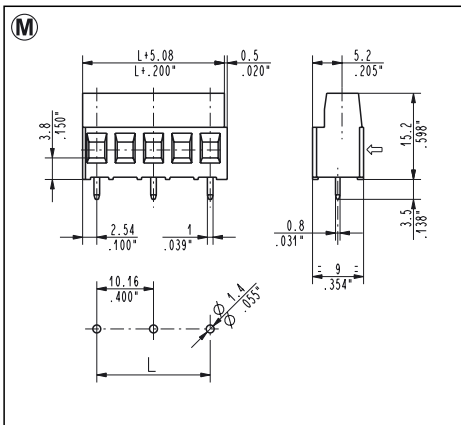
MSM__006 Straight, Side Entry 10.16 mm / .400" Pitch Weight per pole: 1.77 g
