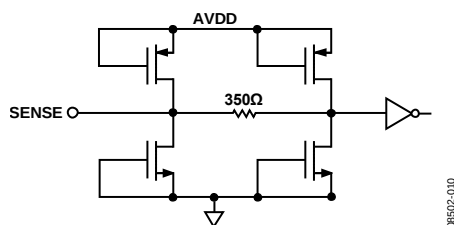
Figure 56. Equivalent SENSE Circuit
