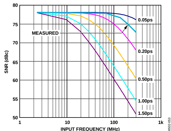
Figure 80. SNR vs. Input Frequency and Jitter
