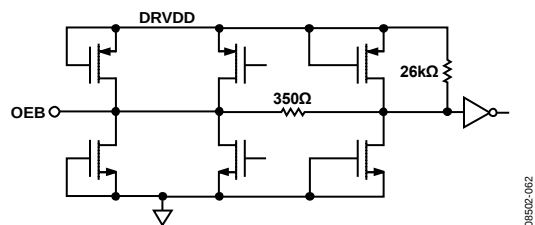
Figure 62. Equivalent OEB Input Circuit
