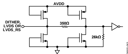
Figure 63. Equivalent DITHER, LVDS, and LVDS_RS Input Circuit
