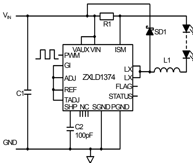
Figure 26 Buck Configuration
