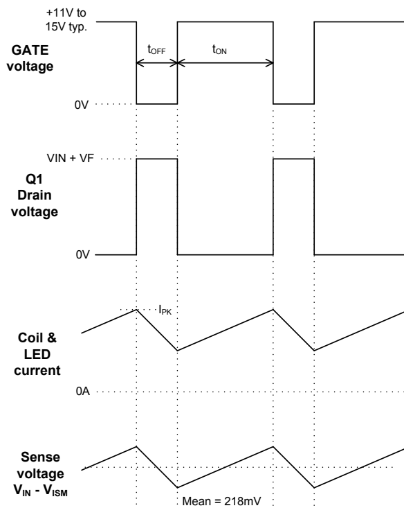
Figure 27 Operating Waveforms (Buck Mode)
