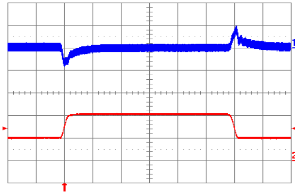
Fig. 1.5V.5: Output voltage response to load current step-change (5 A – 10 A – 5 A) at V_{in} = 48\text{ V} . Top trace: output voltage (100 mV/div.). Bottom trace: load current (5 A/div.). Current slew rate: 0.1 A/ \mu\text{s} . C_o = 1\text{ }\mu\text{F} ceramic. Time scale: 0.2 ms/div.
