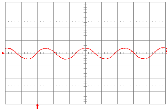
Fig. 2.5V.9: Input reflected ripple current, i_c (100 mA/div.), measured at input terminals at full rated load current and V_{in} = 48 \text{ V} . Refer to Fig. 2.5V.8 for test setup. Time scale: 1 \mu\text{s}/\text{div} .
