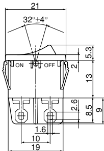
Long guard type Soldering terminal
