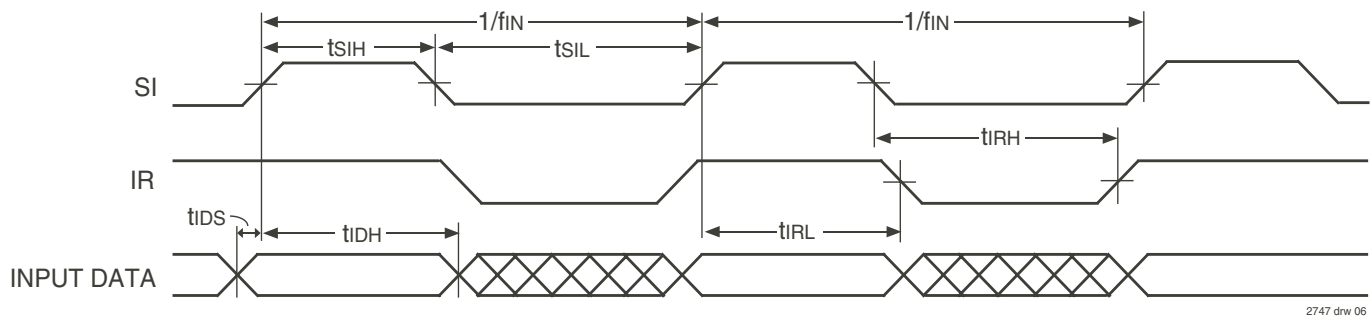
Figure 2. Input Timing
