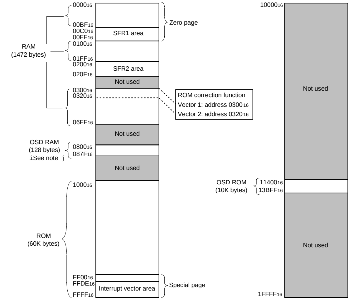
jM37273MF-XXXSP, M37273EFSP
