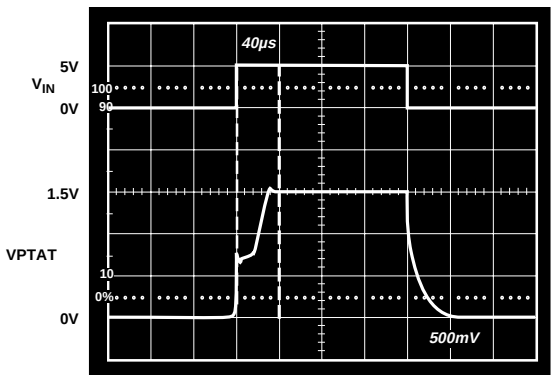
Figure 5. Start-Up Response
