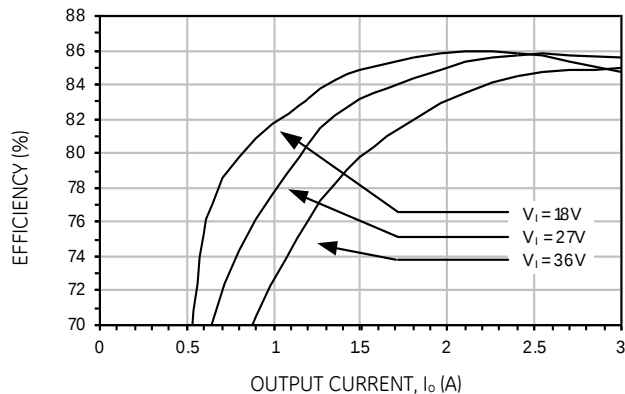
Figure 31. Converter Efficiency Vs Load.
