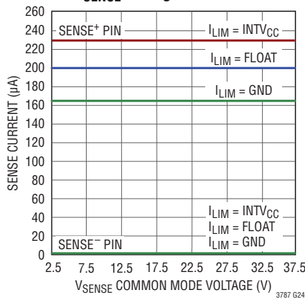
SENSE Pin Input Current vs V_{SENSE} Voltage
