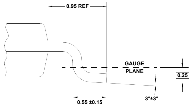
DETAIL "X"
