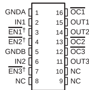
TPS2043A, TPS2053A D PACKAGE (TOP VIEW)
