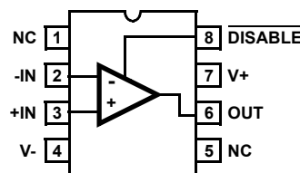
HFA1145 (SOIC) TOP VIEW
