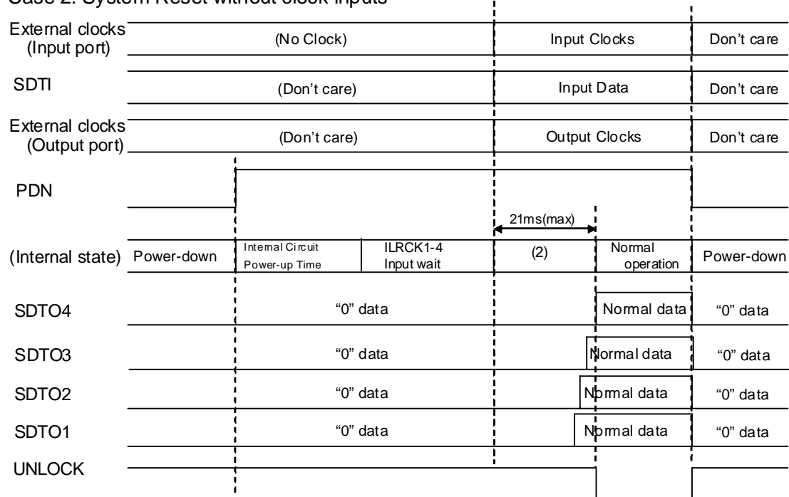
Figure 35. System Reset 2
