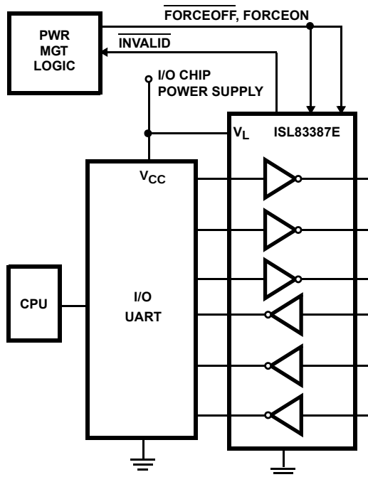
FIGURE 2. CONNECTIONS FOR MANUAL POWERDOWN
