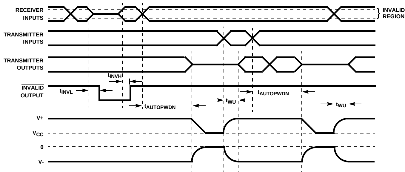
FIGURE 7. ENHANCED AUTOMATIC POWERDOWN AND INVALID TIMING DIAGRAMS
