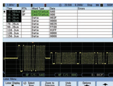
Time-correlated display of the MIL-STD 1553 physical layer signal with protocol decoding.
