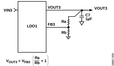
Figure 48. LDO1 External Output Voltage Setting
