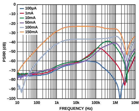
Figure 41. LDO PSRR Across Output Load, V_{IN3} = 3.3\text{ V} , V_{OUT3} = 2.8\text{ V}
