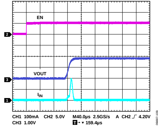
Figure 30. LDO Startup, V_{OUT3} = 1.8 V
