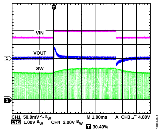
Figure 24. BUCK2 Response to Line Transient, V_{IN2} = 4.5\text{ V} to 5.0\text{ V} , V_{OUT2} = 1.8\text{ V} , PWM Mode
