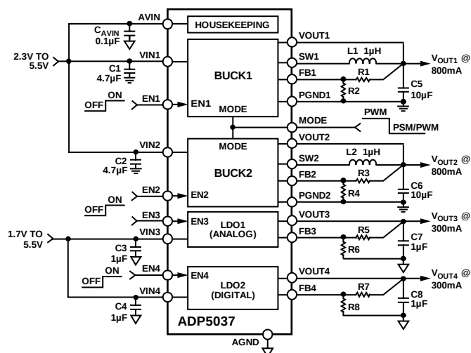
Figure 53. ADP5037 Adjustable Output Voltages with Enable Pins
