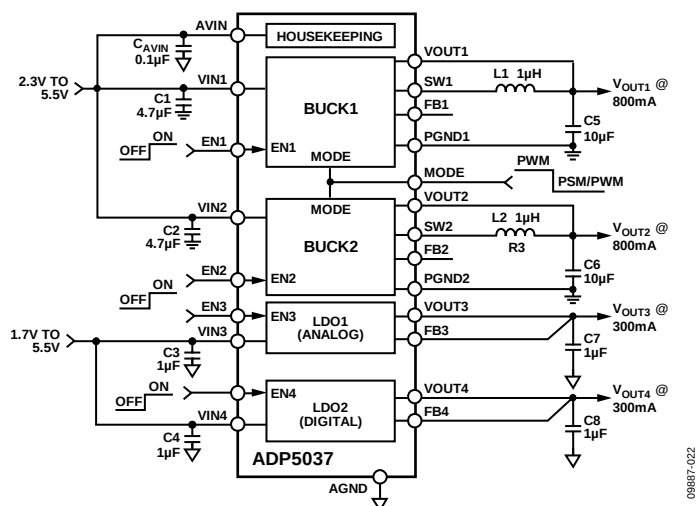
Figure 52. ADP5037 Fixed Output Voltages with Enable Pins
