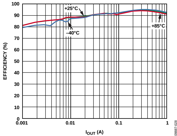
Figure 15. BUCK1 Efficiency vs. Load Current, Across Temperature, V_{IN} = 3.9\text{ V} , V_{OUT1} = 3.3\text{ V} , Auto Mode
