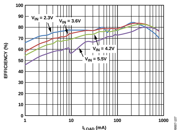
Figure 13. BUCK1 Efficiency vs. Load Current, Across Input Voltage, V_{OUT1} = 0.8\text{ V} , Auto Mode
