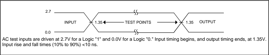
Figure 12. Transient Input/Output Reference Waveform for V_{CC} = 2.7V-3.6V
