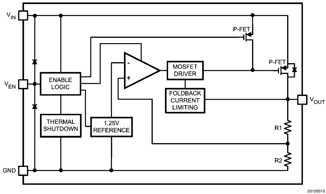
FIGURE 4. LP38693 Functional Diagram (SOT-223)
