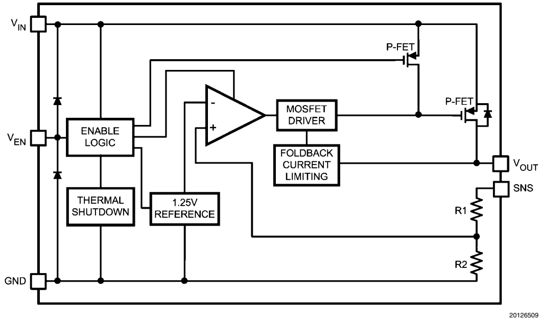
FIGURE 3. LP38693 Functional Diagram (LLP)
